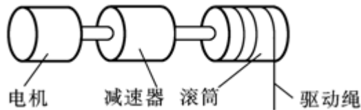
(a) 减速器滚筒驱动
